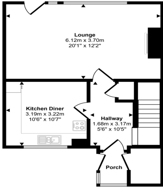
Ground Floor Approx 48 sq m / 513 sq ft
